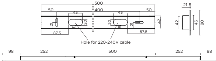
12.0 - back plate and luminaire dimensions
