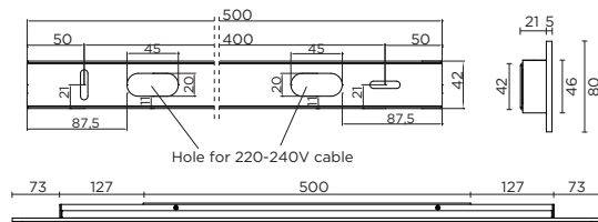
9.0 - back plate and luminaire dimensions
